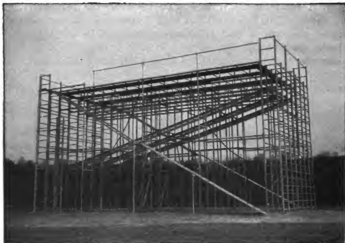
FIGURE 31. —Metal trainer or train trestle.
